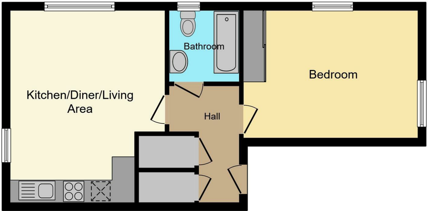
Floor Plan
